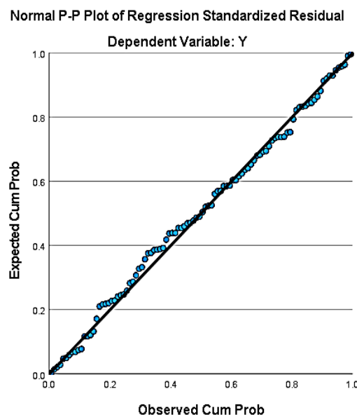
Figure 1. Scatter Plot
